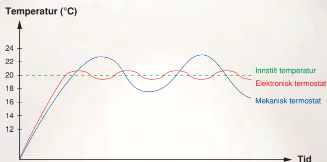
Prinsippkisse for termostatregering
